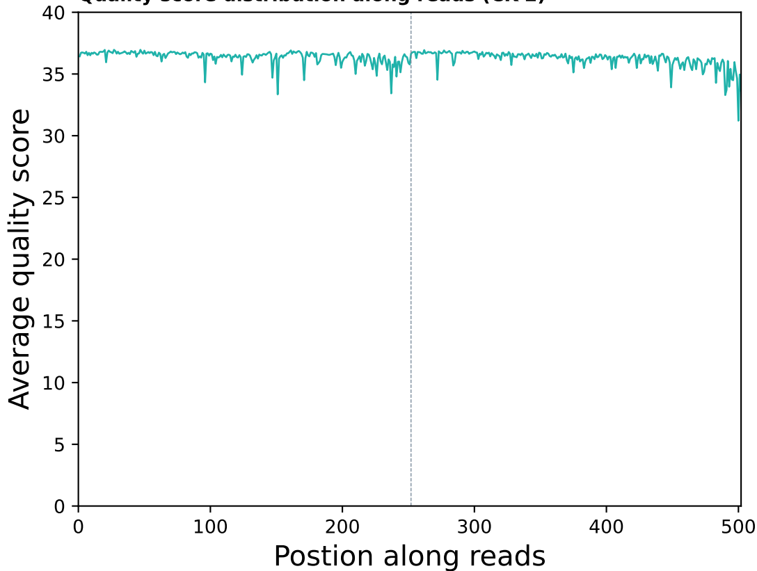
Quality score distribution along reads (CK-2)
